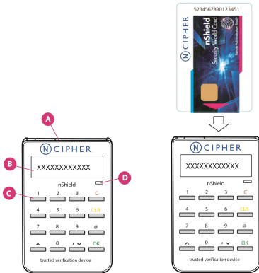
Figure 4. The nShield TVD controls, card slot, and LED
