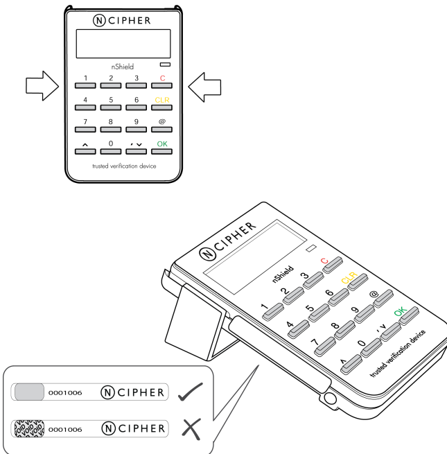
Figure 1. nCipher tamper seals
